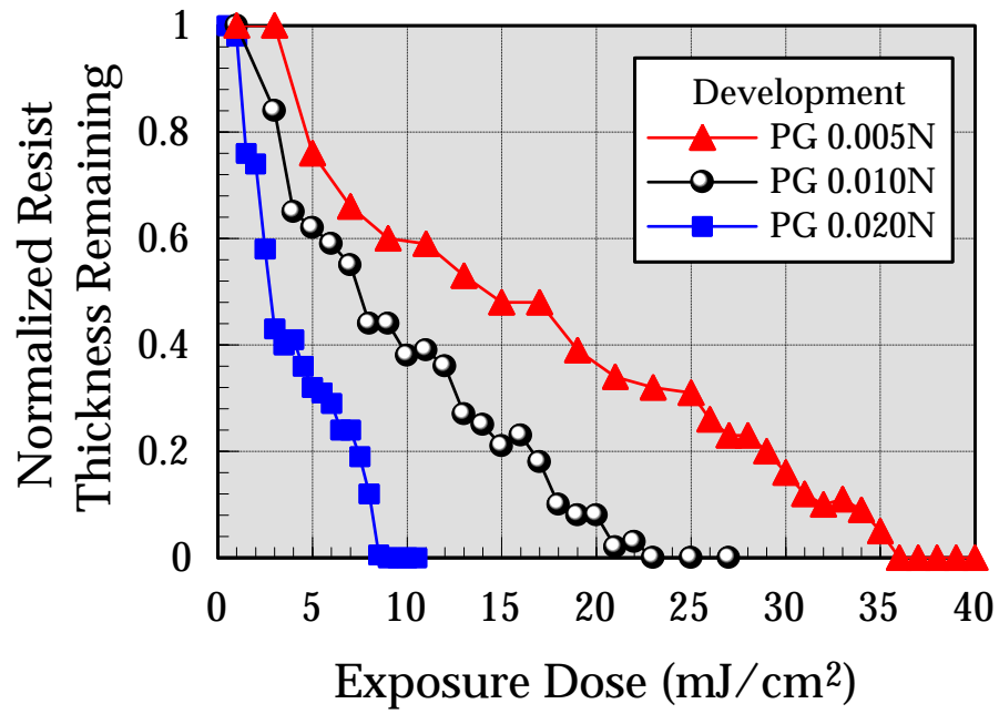
Figure 7. Contrast curve for TER-1 at 193nm
