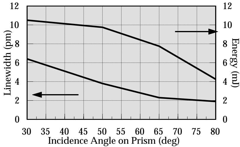
Figure 4. Performance of line-narrowed excimer laser with prism beam expansion.
