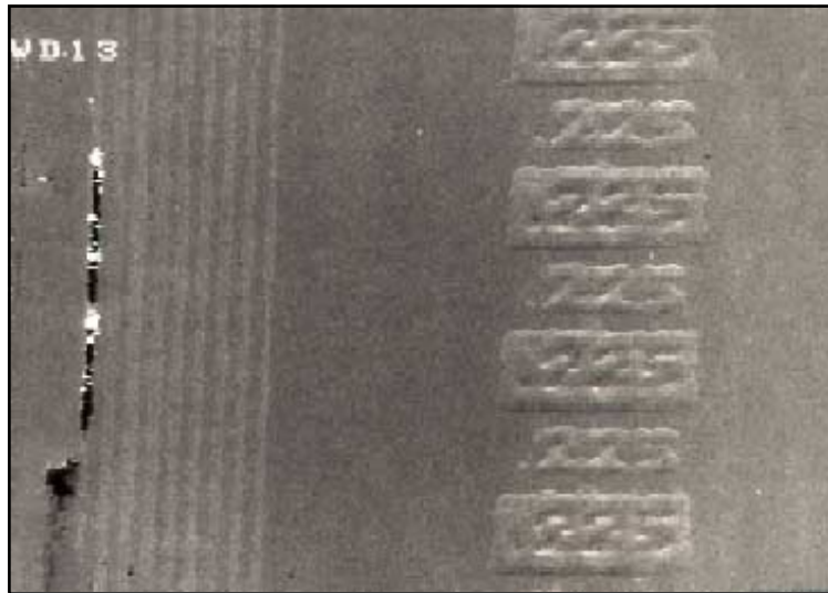
Figure 8. Dense lines and spaces in TER-1 (under-developed)
