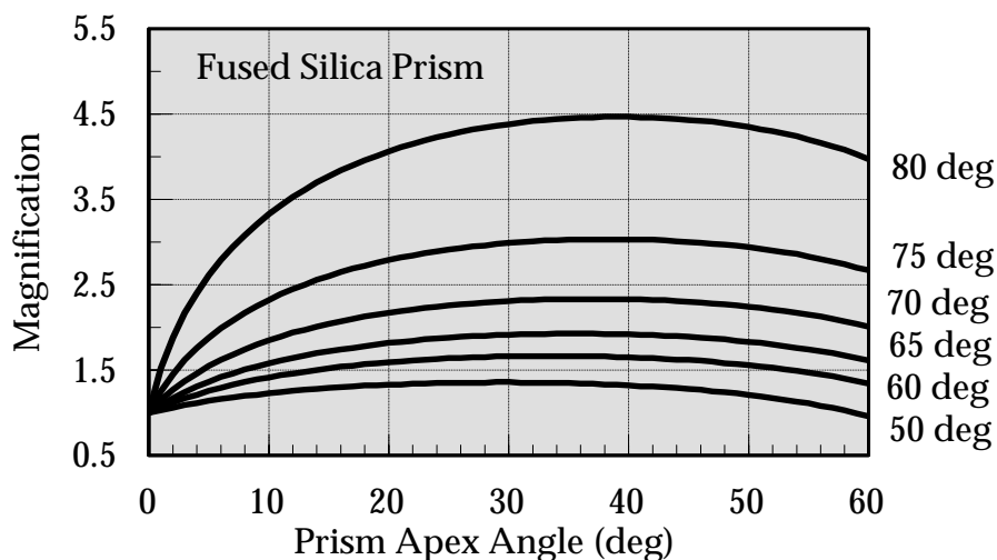
Figure 3. Prism beam expansion for different incidence angle on prism for line-narrowing.
