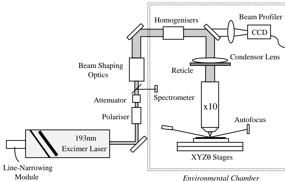
Figure 2. Schematic diagram of 193nm Microstepper
