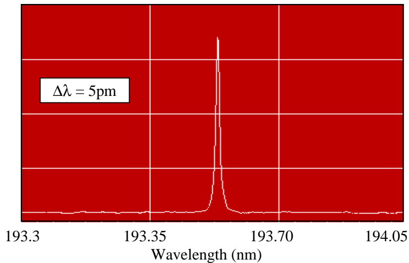
Figure 5. Line-narrowed spectrum.
