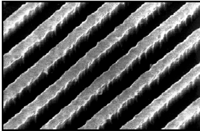
Figure 6. 0.2 \mu m lines and spaces in MX-P8 exposed at 193nm
