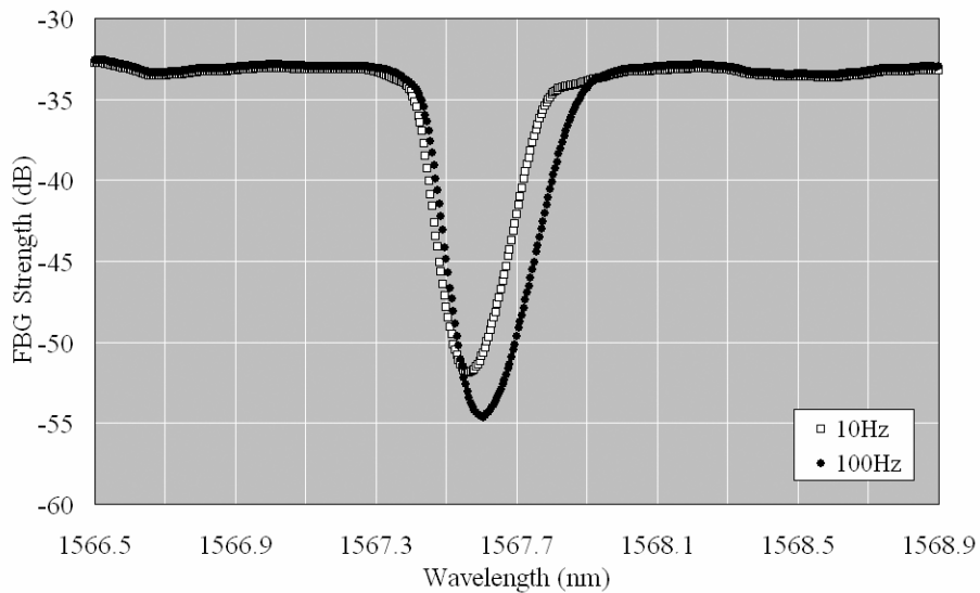
Figure 6. FBG spectra obtained with increasing laser repetition rate, with all other exposure parameters being fixed.
