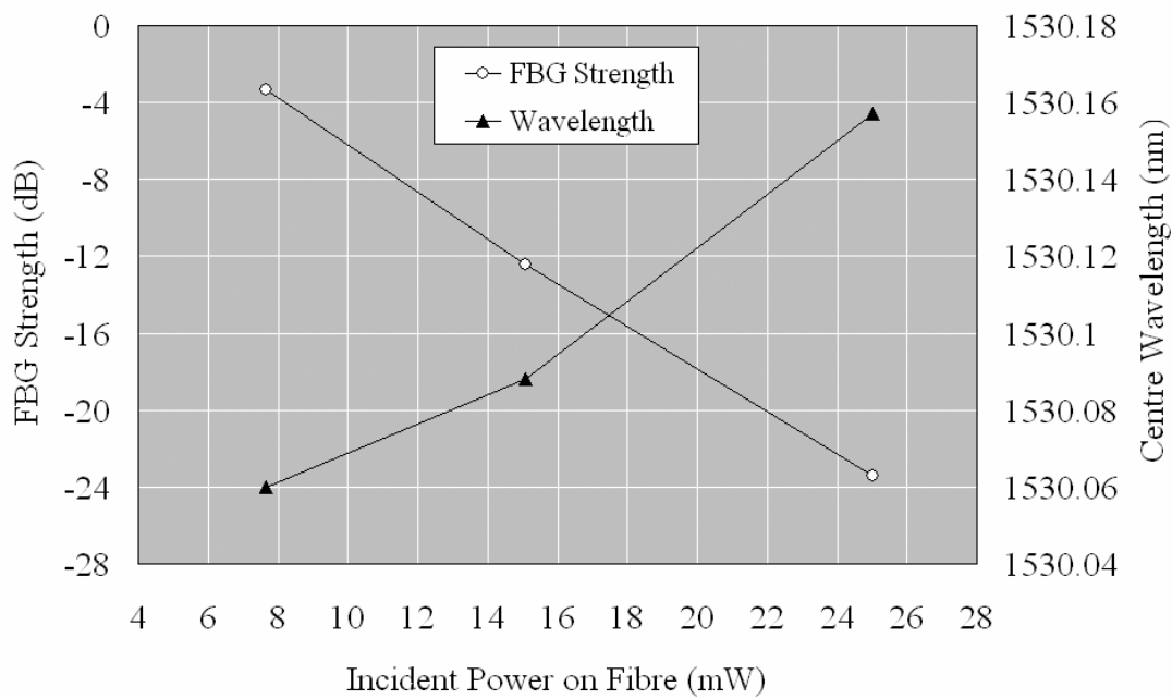
Figure 10. Variation of the strength and centre wavelength of FBGs for different beam powers from an argon ion laser.
