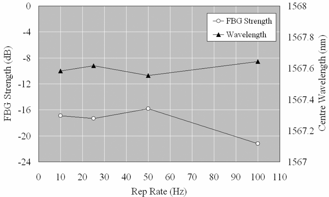
Figure 5. Variation of FBG strength and centre wavelength versus laser repetition rate for fixed exposure conditions.
