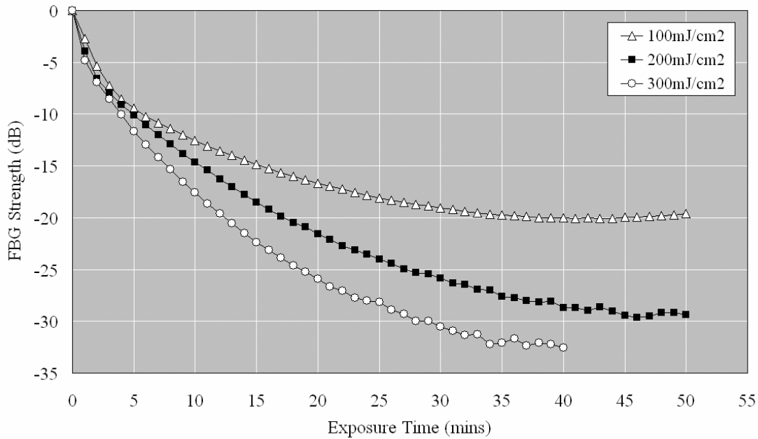
Figure 4. Variation in grating strength with increasing exposure times for three exposure fluences.
