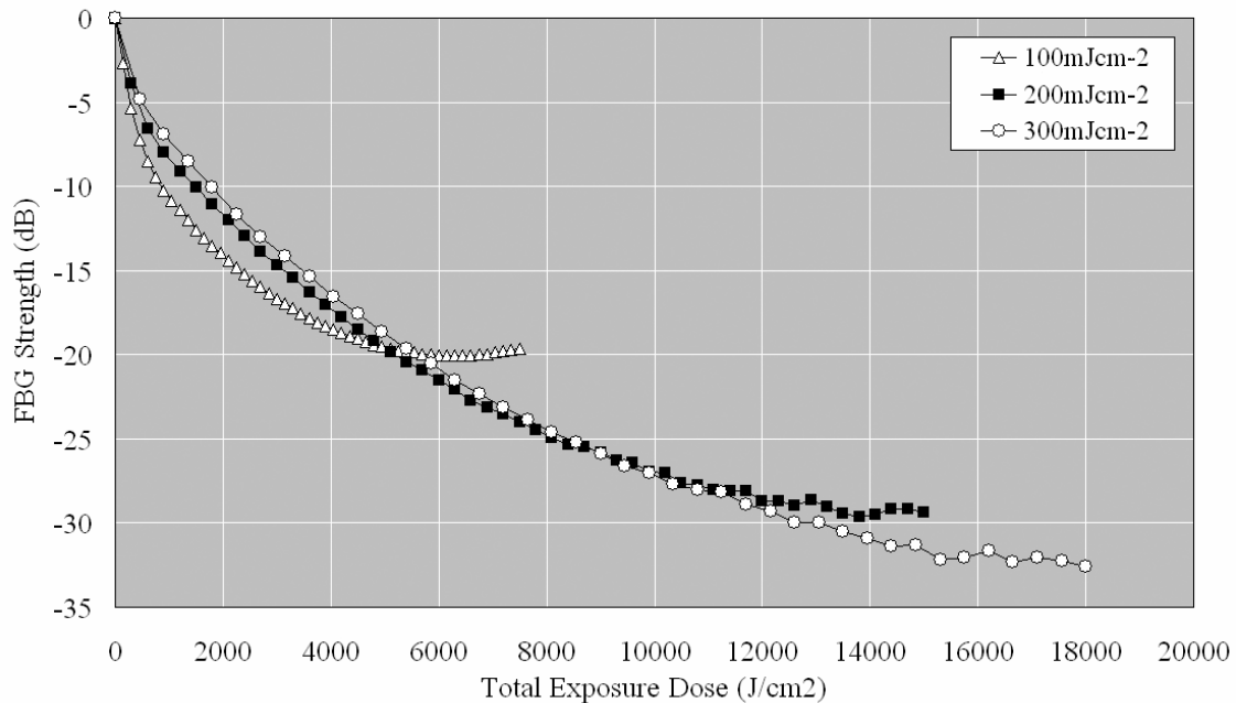
Figure 3. Variation of grating strength with increasing dose for three exposure fluence levels.
