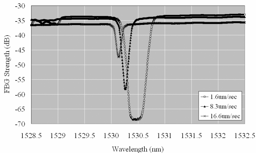
Figure 9. Transmission spectra of gratings produced with varying scan speeds using an argon ion laser.
