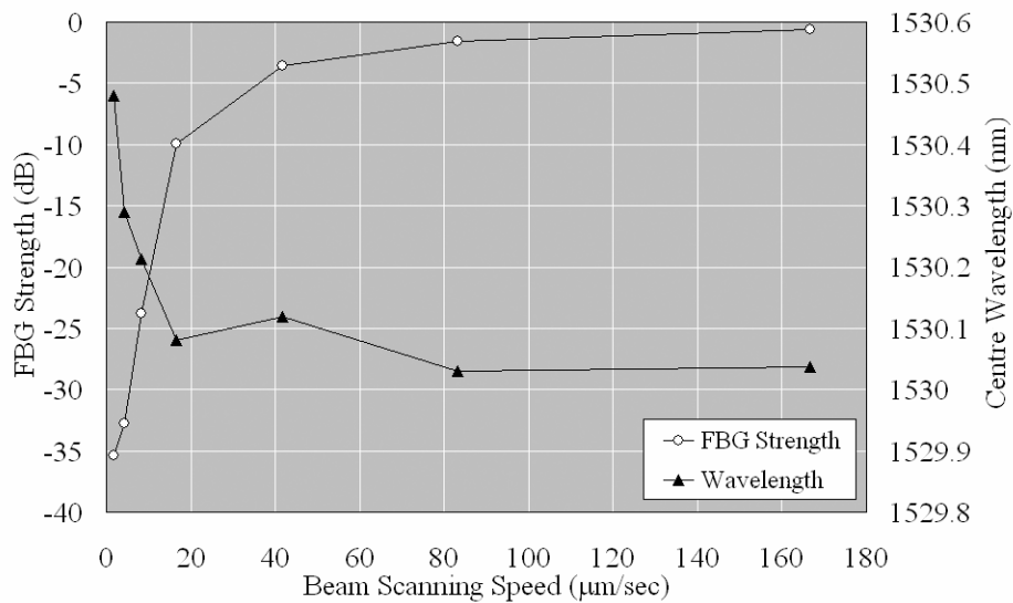
Figure 8. Variation of the strength and centre wavelength of FBGs for different beam scanning speeds from an argon ion laser.
