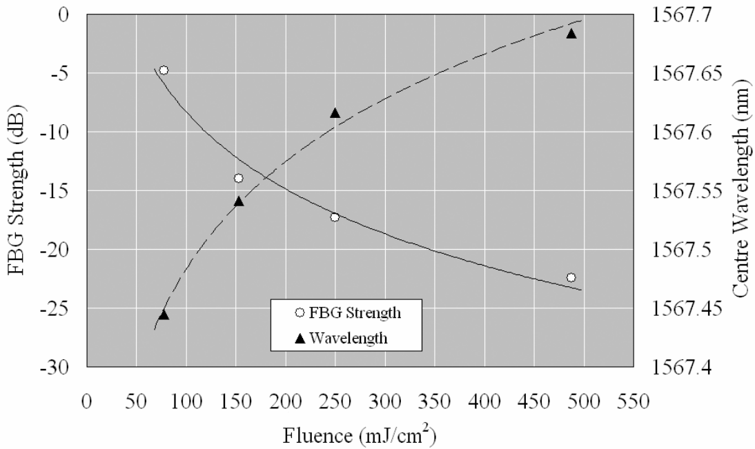
Figure 1. Graph showing variation in the strength of FBGs in H-loaded SMF28 fibres versus exposure fluence.
