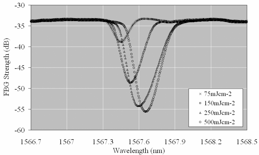
Figure 2. Spectral evolution of FBGs as exposure fluence is increased for a fixed dose.
