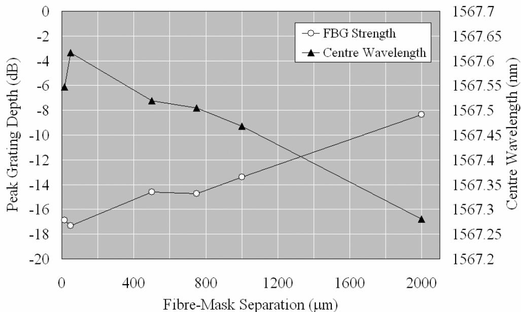
Figure 7. Variation of FBG strength and centre wavelength versus fibre-mask separation for fixed exposure conditions.
