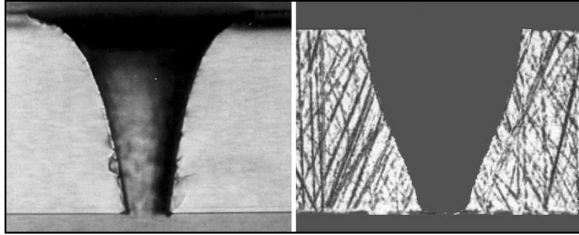
Figure 4. Shaped nozzle cross-sections in glass (left) and polycarbonate (right) drilled using excimer lasers.
