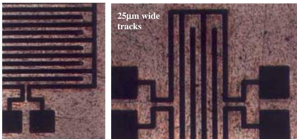
Figure 7. Circuit patterns ablated into polyimide (on copper substrate) by 3 rd harmonic Nd:YAG laser.
