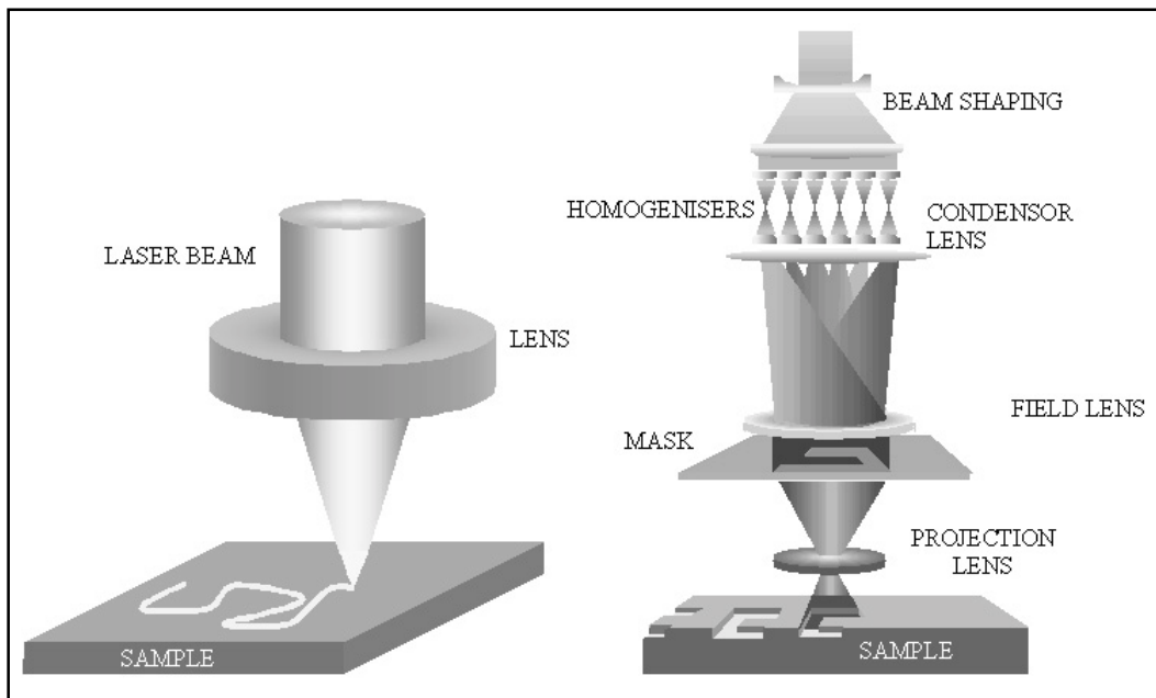
Figure 1. Representation of (a) direct writing and (b) mask projection.
