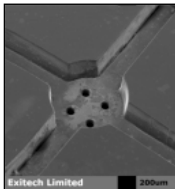
Figure 3. Nozzles machined in polyimide using multiple mask projection.
