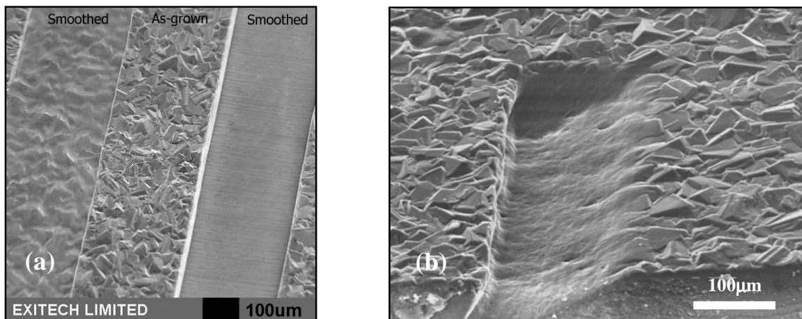
Figure 9. Laser smoothing of CVD diamond using (a) an excimer laser at 248nm and (b) a femtosecond Ti:sapphire laser at 800nm.
