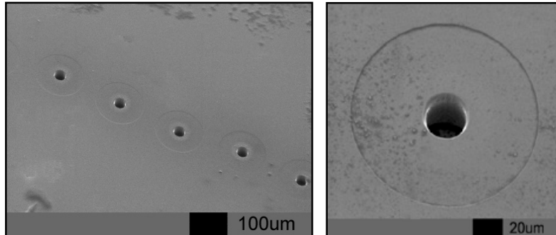
Figure 2. Ink-jet printer nozzles drilled using excimer laser mask projection.
