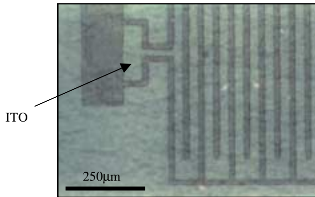
Figure 6. ITO layer on glass patterned with 355nm Nd:YAG laser.
