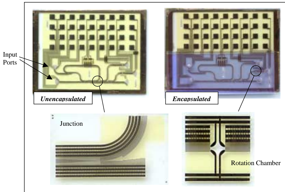
Figure 8. Biochip manufactured using laser micromachining.
