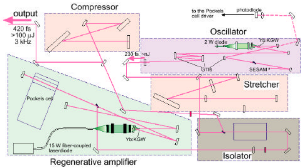
Fig. 2: Set-up of the diode-pumped fs laser system
