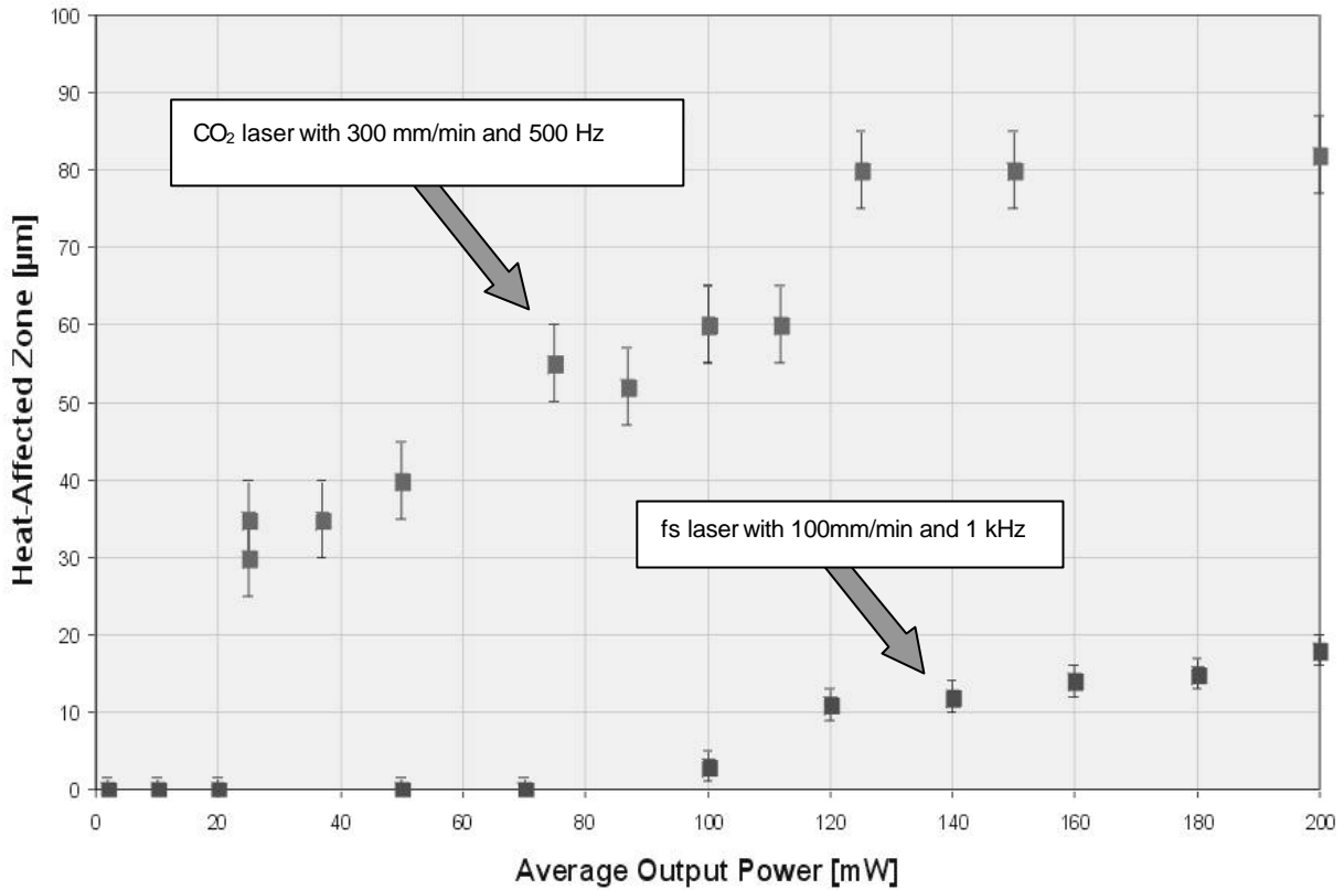
Fig.6: Diagram of heat-affected zones in biodegradable polymers of CO 2 and fs laser machined cuts.
