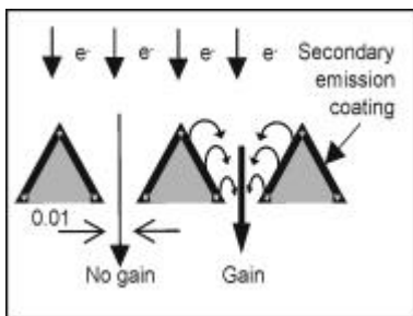
Fig. 5a: Optimal cross-section of the dynode structure
