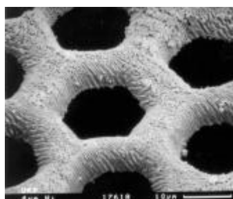
Fig. 5b: Detail of the hexagonal dynode structure, Periodicity of 23\ \mu\text{m} .
