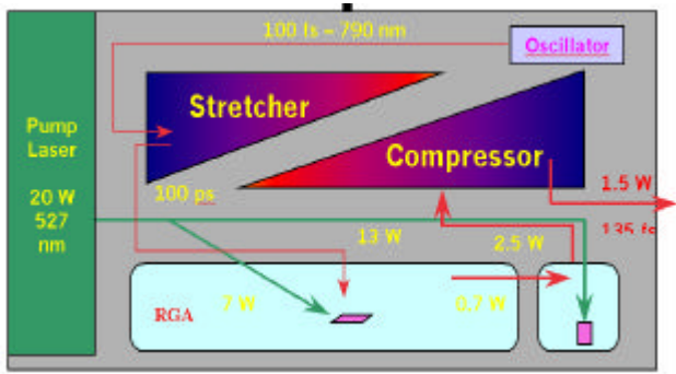
Fig. 1a: Schematic of the set-up of the ti:sapphire amplifier
