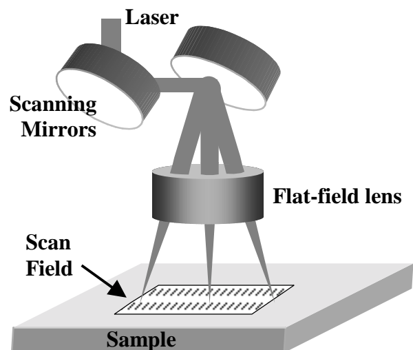
Figure 7. Technique of direct writing.
