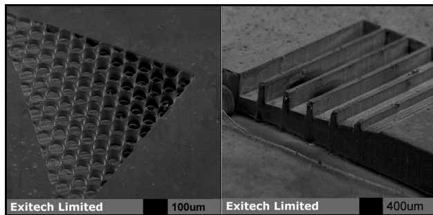
Figure 6. Demonstration of multi-level micro-structuring using synchronised overlay scanning.
