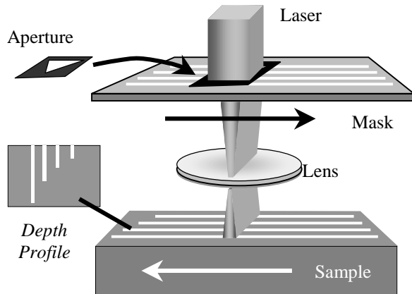
Figure 3. Technique of synchronised overlay scanning.
