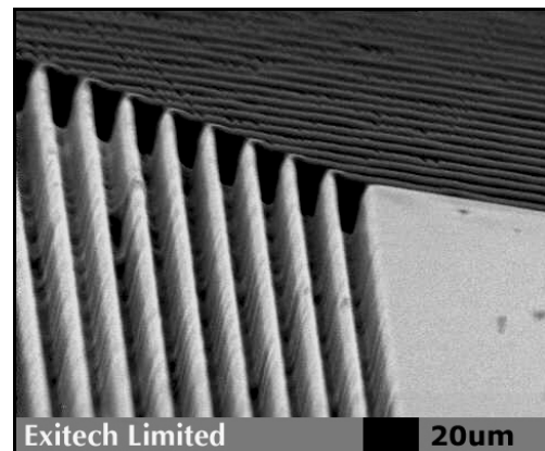
Figure 2. Micro-channels produced by mask projection in polymer showing depth control.
