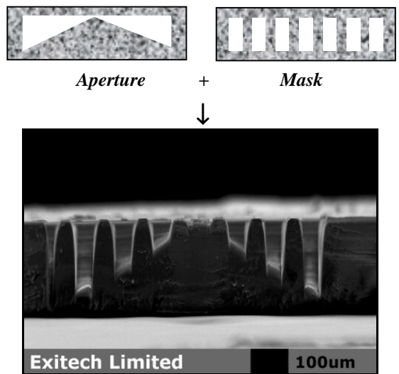
Figure 5. Micro-channels on double ramp in PET.
