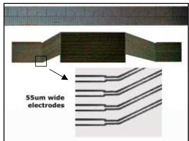
Figure 8. Electrical inter-connect structures for display devices patterned using direct writing with Sync Scan.
