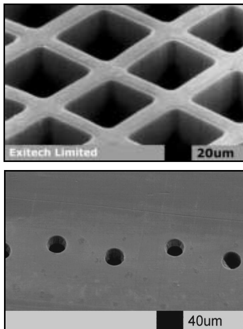
Figure 1. (a) Micro-machining of polyimide and (b) ink-jet printer nozzles, both produced using excimer laser mask projection.
