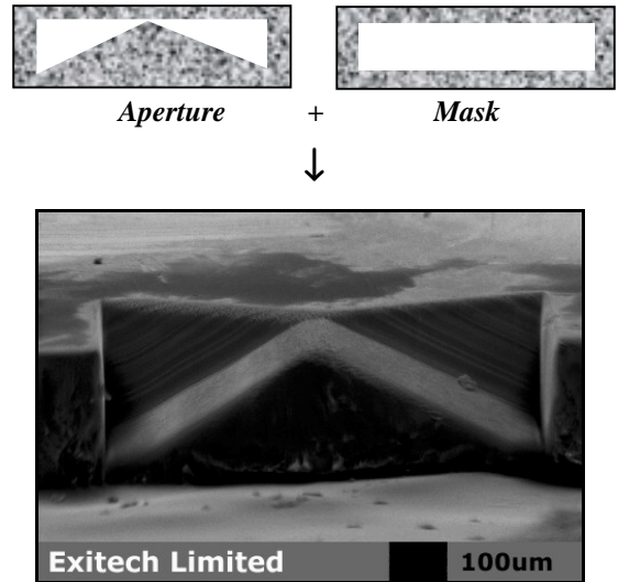
Figure 4. Double ramp produced in PET.
