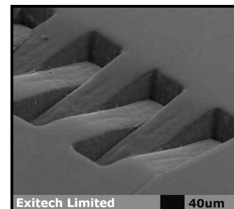
Figure 7. Multiple ramp structures produced in polymer by moving mask technique. The ramps of one direction are produced at the same time followed by the ramps of the other direction.
