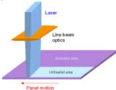
Figure 11. Excimer laser annealing where the panel is moved in a raster fashion across a line beam.
