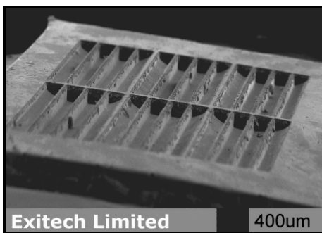
Figure 10. Microchannels produced inside curved wells by synchronised overlay scanning.
