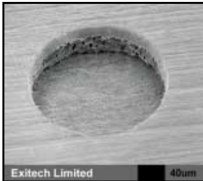
Figure 4. Hole trepanned into top copper layer using a Nd:YAG laser. Also visible is a central polymer layer which has been machined with a CO 2 laser and the base copper layer which is undamaged.
