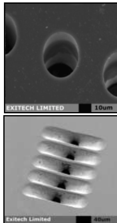
Figure 12. Nozzle holes in polyimide made with excimer lasers
