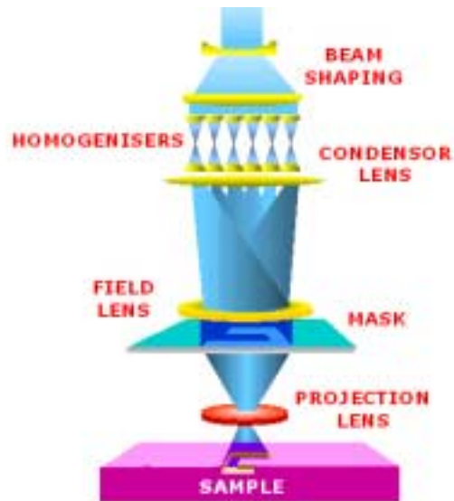
Figure 5. Schematic diagram excimer laser mask projection system.
