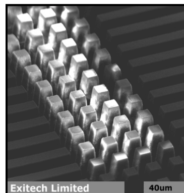
Figure 15. Micro-optical structures produced by excimer laser mask projection and workpiece motion technique.
