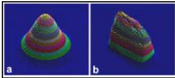
Figure 2. Typical beam profiles showing differences in mode structure from (a) Nd:YAG laser (b) excimer laser.
