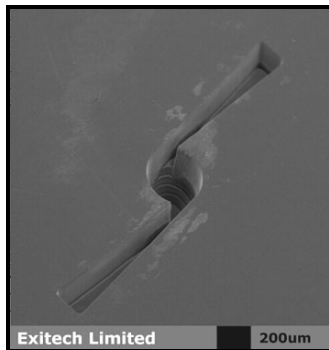
Figure 16. Micro-fluidic device incorporating multi-level excimer laser micro-machined structures.
