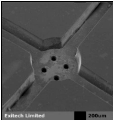
Figure 13. Micro-holes drilled into polymer reservoir for a micro-fluidic device.
