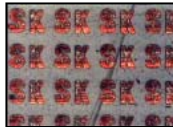
Figure 6. Polymer layer on copper selectively removed by laser ablation. The 120 \mu m high "SK" characters are produced by step-and-repeat processing.
