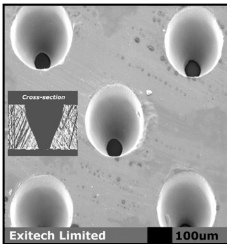
Figure 14. Tapered holes produced by excimer laser mask projection with sample motion. A cross-section of the holes is shown in the inset.
