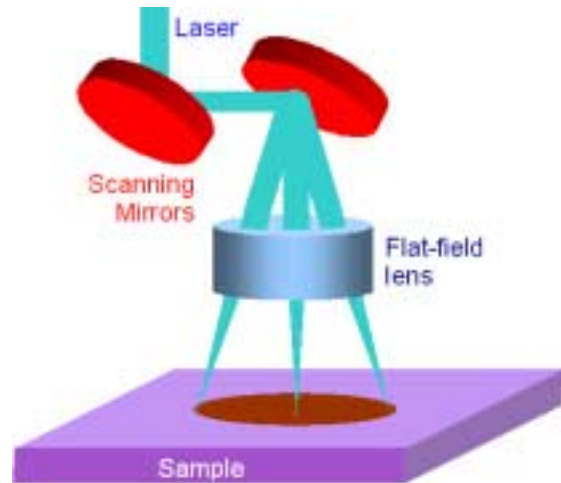
Figure 3. Schematic diagram of beam scanning technique where galvanometer-driven mirrors deflect the laser beam to the desired locations for micromachining.
